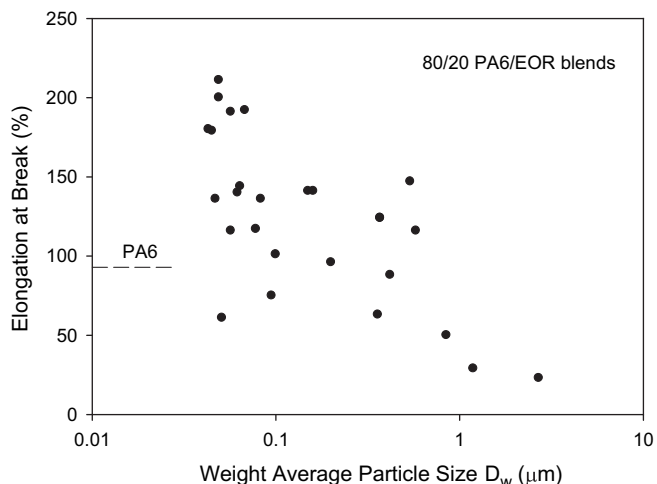
Fig. 9. Tensile elongation at break of dry PA6 blends containing 20% by weight of ethylene-octene rubber. Data of Huang et al. [2].
