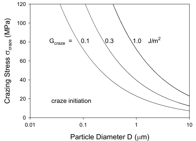
Fig. 7. Critical tensile stress for craze initiation as a function of (cavitated) rubber particle diameter, calculated using equation (16) with three different values of G_{\text{craze}} , the specific energy of craze initiation.
