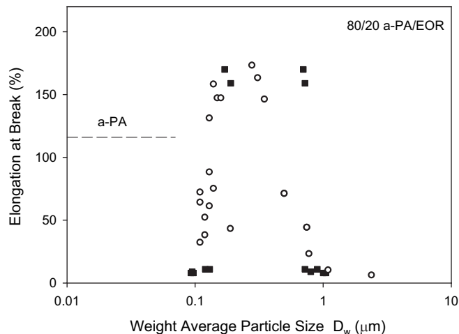
Fig. 10. Tensile elongation at break of dry a-PA blends containing 20% by weight of ethylene-octene rubber. Data of Huang et al. [2]. Open circles denote blends with monodisperse particle size distribution. Closed squares denote bimodal distributions, with each blend represented twice, to show upper and lower peaks in the size distribution separately.
