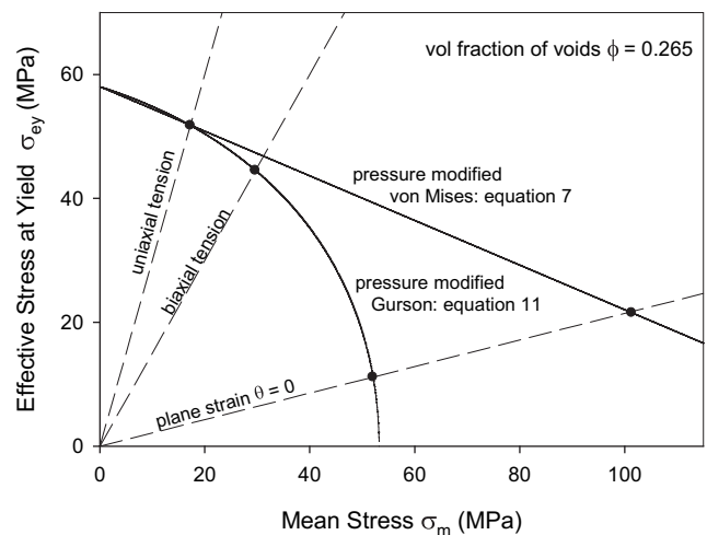
Fig. 4. Comparison between pressure-modified von Mises criterion for a void-free blend (equation (7) with \mu = 0.36 ) and pressure-modified Gurson criterion for the same blend, now fully-cavitated (equation (11)).
