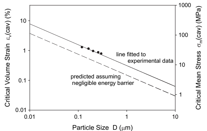
Fig. 2. Effect of rubber particle size on critical volume strain and critical mean stress at cavitation. Data obtained by Dompas et al in tests on transparent PVC/MBS blends [46]. Dotted line calculated using energy balance model, equation (6), with \varepsilon_v constant. Solid line is parallel to dotted line, but shifted upwards by a factor of 2.1 to fit data.
