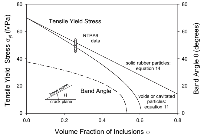
Fig. 5. Effect of low modulus inclusions (voids or solid rubber particles) on tensile yielding in dry PA6, and of voids on band angle (alternating dashes and dots)[68]. Data points from Huang et al. [2].
