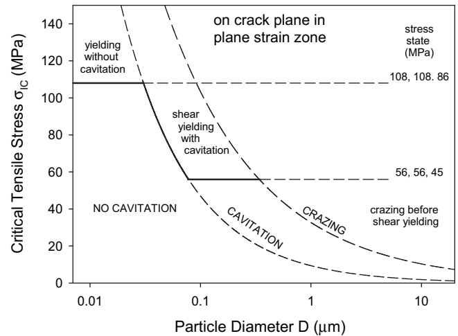
Fig. 11. Schematic diagram illustrating effects of particle size on deformation mechanisms close to the crack plane ( \theta = 0 ) under plane strain conditions, in 80/20 RTPA6 blends. Craze line calculated using equation (16) with E = 2.8 GPa and G_{\text{craze}} = 0.2 J/m 2 . Shear yield stresses calculated using equation (7), with pressure coefficient \mu = 0.36 (see Fig. 4). Solid line defines critical stress for shear yielding, both with and without prior cavitation. Note that crazing and shear yielding can take place simultaneously in tough specimens containing relatively large particles.
