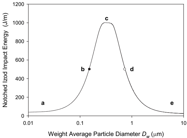
Fig. 1. Relationship between particle size and impact behaviour for a typical ‘supertough’ thermoplastic blend. Points b and d mark lower (●) and upper (○) ductile–brittle transitions. Schematic representation based broadly on data of Huang et al. for a series of 80/20 RTPA6 blends [2].
