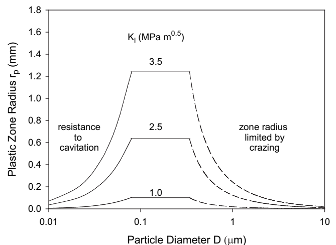
Fig. 12. Plane strain plastic zone radius at \theta = 0 , calculated using equation (3) with r_p doubled (Irwin’s correction factor [64, 66]). Yield stress data taken from Fig. 11, on the assumption that the shear yield zone is fully developed. At large particle sizes, craze formation increases the probability that the specimen fails through crack initiation in regions of high local stress. Dotted lines are estimates based very roughly on observed reductions in fracture resistance of notched specimens.
