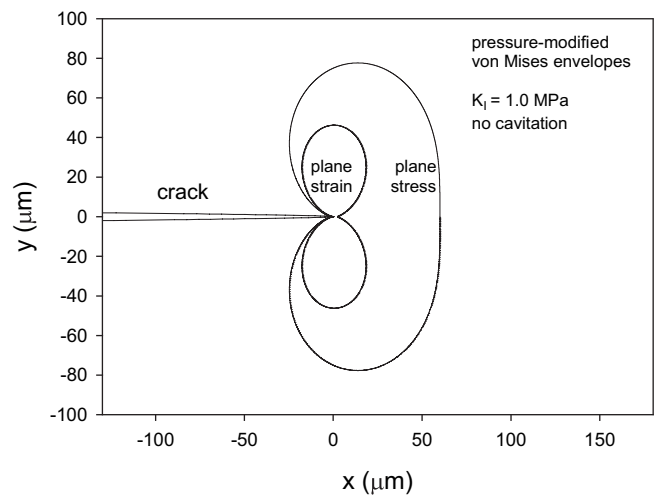
Fig. 6. Pressure-dependent von Mises yield envelopes under plane stress and plane strain loading, with K_I = 1.0 MPa m^{0.5} , for void-free 80/20 PA6/rubber blend with Poisson's ratio \nu = 0.4 , pressure coefficient \mu = 0.36 .
