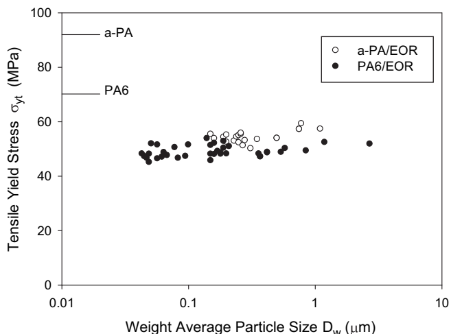
Fig. 8. Yield stresses of dry 80/20 a-PA and PA6 blends over a range of particle sizes at 23 °C. Horizontal lines indicate yield stresses of neat a-PA and PA6 in dry state. Data of Huang et al. [2].
