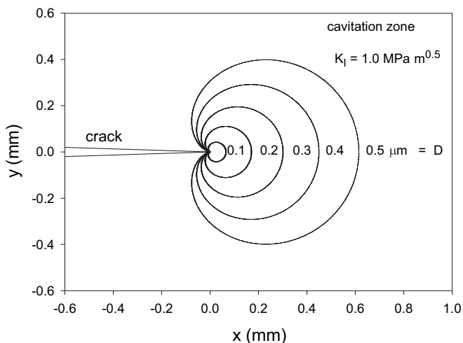
Fig. 3. Map of cavitated zone in plane strain region, showing dependence of zone boundary on particle diameter when K_I = 1 MPa m 0.5 . Critical mean stresses calculated using equations (2a)–(2d) with bulk modulus K_b = 3 GPa and data from solid curve in Fig. 2.
